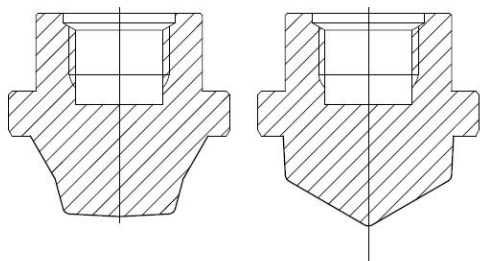
Control plug equal percentage
