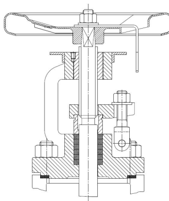
position indicator
