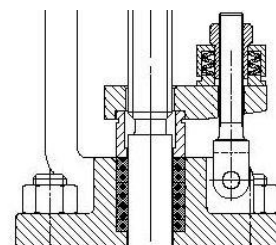
spring load system
