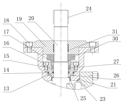
GP(Gland, PTFE)
