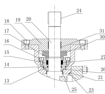
GG(Gland, Graphite)
