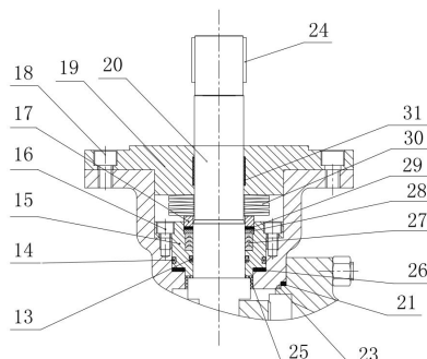
GPG(Gland, PTFE+Graphite)
