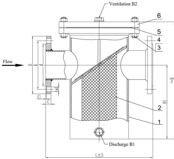
Basket type strainers
