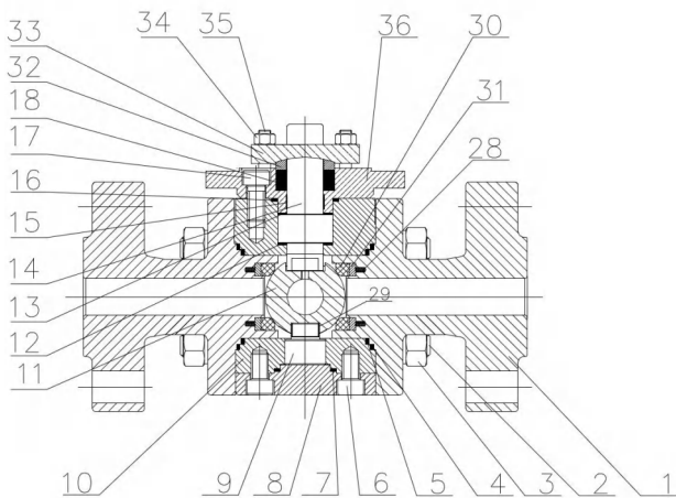
DN65 - DN300 Graphite Packing fire safe
